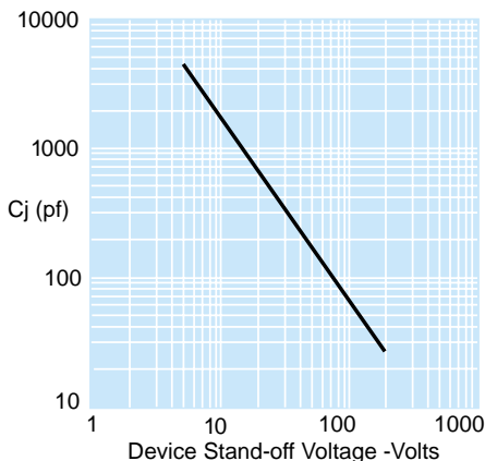
Figure 1 - Capacitance vs. Stand-off Voltage
