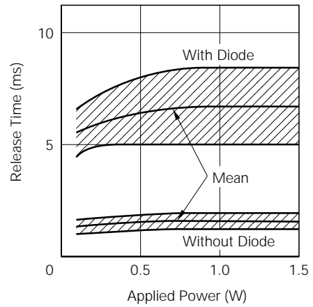
Release time (EP2-3L1)
