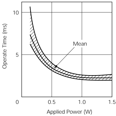
Operate Time (EP2-3L1)
