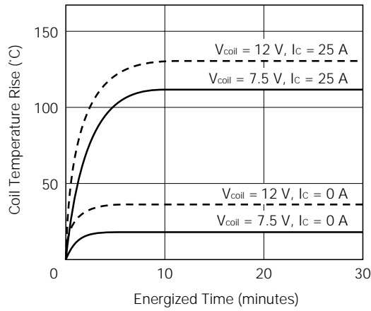
Coil Temperature Rise (EP2-3L1)
